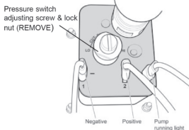
Fig 2 Wiring connections Watermaster socket
