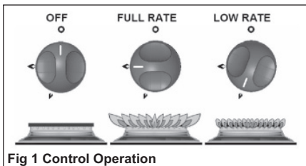
Fig 1 Control Operation
