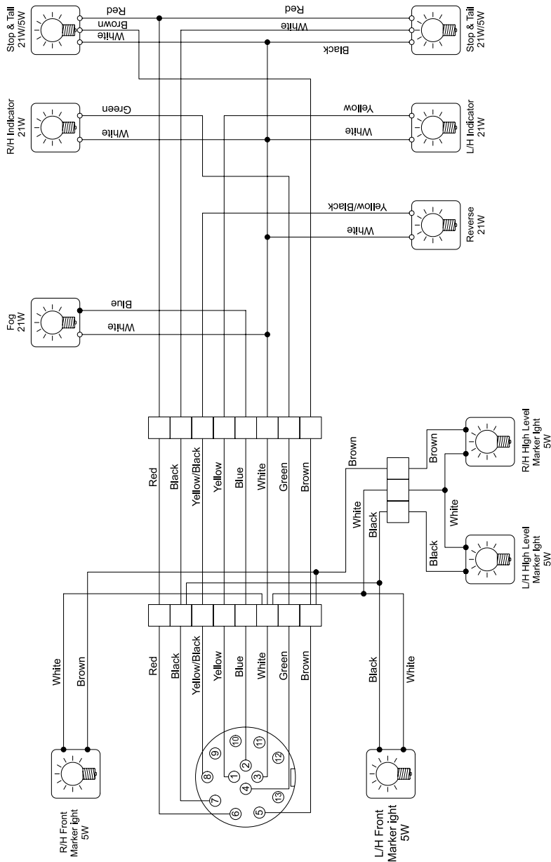
Avante Road Lights Diagram
